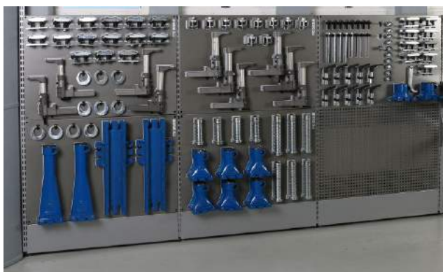
EVO 3-4 For secure holding and anchoring of Jaguar/Land Rover/Range Rover vehicles
